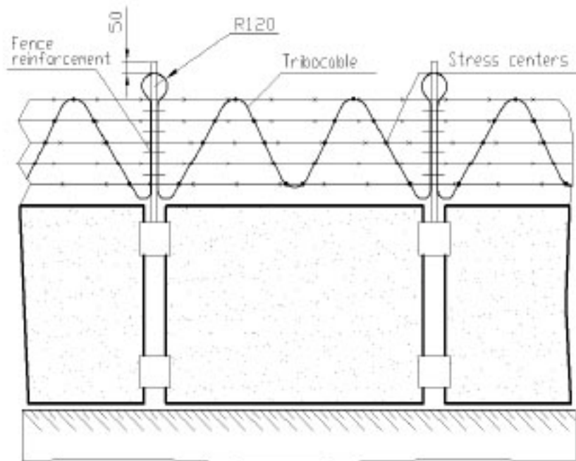
Fig. 2e Extra Barbed-Wire Fence
