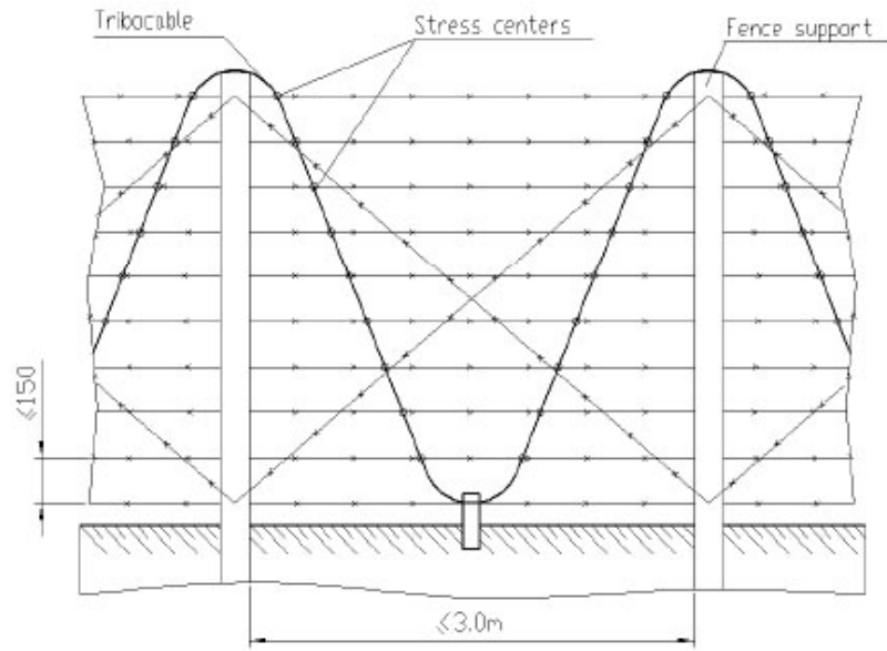
Fig. 1d Barbed-Wire Fence
