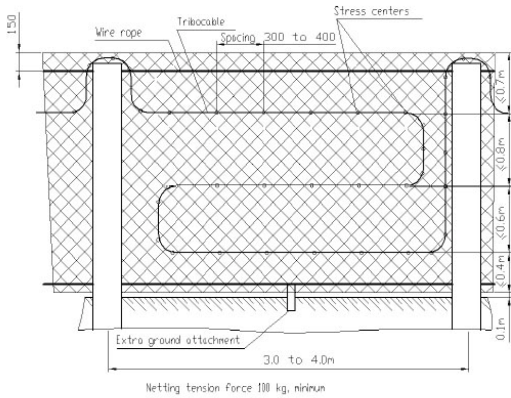
Fig.1b "Rabitsa" Wire-Netting Fence
