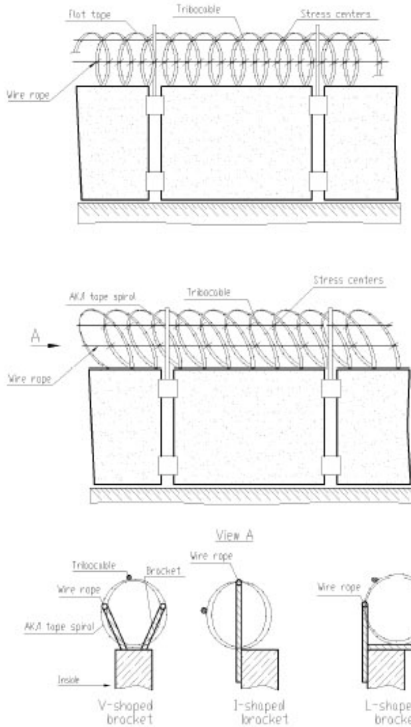
Fig.2e, continued Extra Fence of Spiral or Flat Barbed Tape
