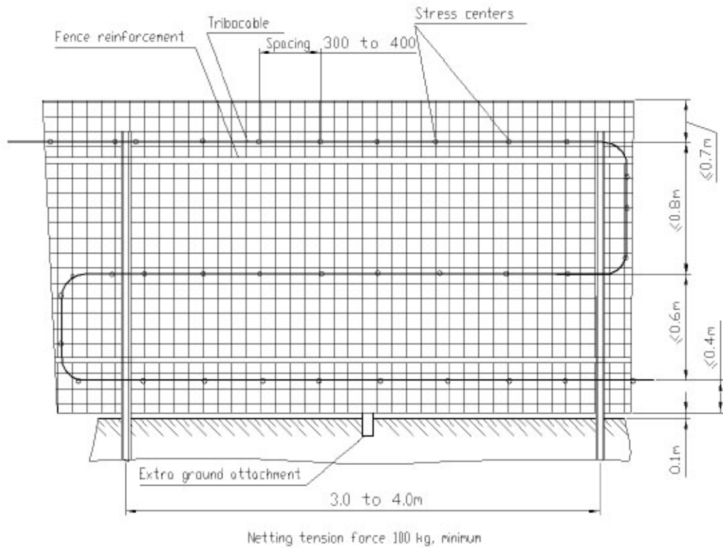
Fig.1a ССЦП Wire-Netting Fence
