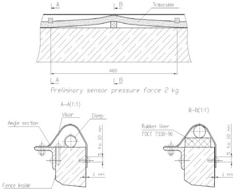
Fig.2d Fence with Visor
