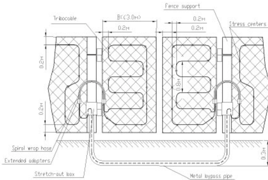
- Fig.3 - Gate (Wicket) Equipping
