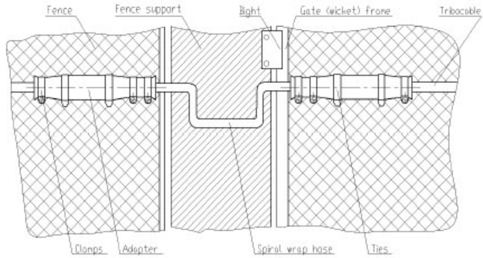
Fig.3a Spiral Wrap Hose Mounting in Extended Adapter
