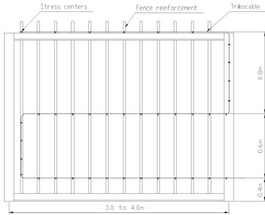
Fig. 2a Fence of Welded (Forged) Gratings
