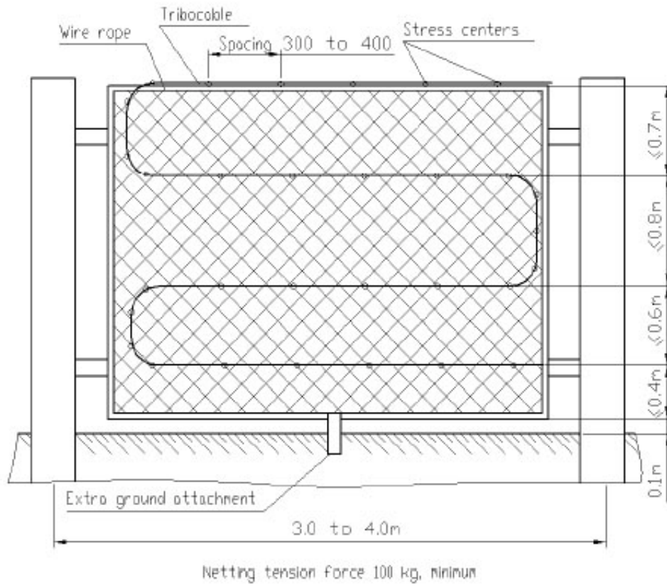
Fig.1c "Rabitsa" Wire-Netting Fence
