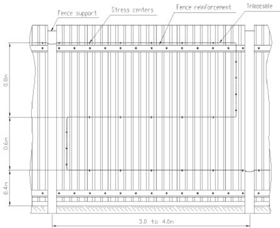
Fig. 2b Fence of Solid Metal Plates
