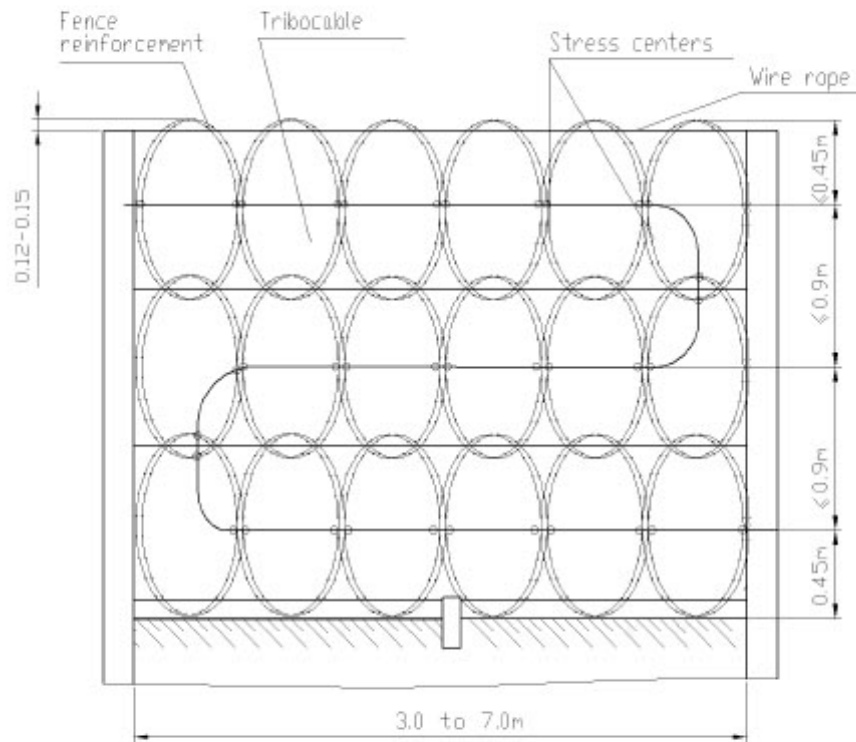
Fig.1e Fence of Reinforced Barbed Tape (AK/A)
